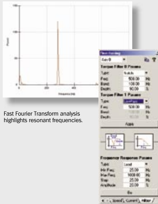
Mint Workbench digital filter design tool.
