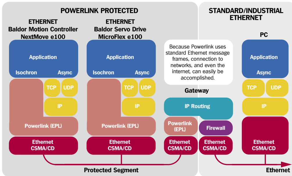
Block diagram showing a Powerlink protected network segment connected to a standard Ethernet network via an EPL gateway/router with integrated firewall.
