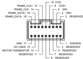
Absolute Encoder
